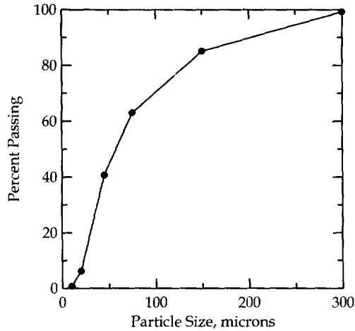
FIG. 1. Particle size distribution of copper slag.
