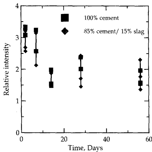
FIG. 9. Variation of alite/belite in slag/cement pastes.
