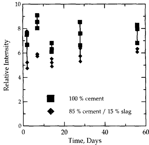
FIG. 8. Variation of CH in slag/cement pastes.
