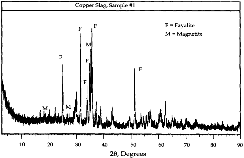
FIG. 2. XRD pattern of a sample of as-received copper slag.
